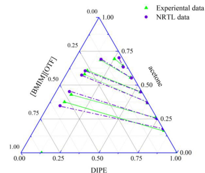
Fig. 2. Experimental and regression data of DIPE + acetone + [BMIM][OTF] at 101.325 kPa and 298.15 K. (▲—), experimental data; (●—), NRTL regression data.
